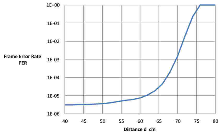
MOL81 1354 / OMR system Frame Error Rate versus distance d
