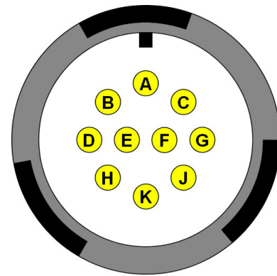
VGE1 type connector from Souraiu Pin side view of the male receptacle or wiring side view of the female plug
